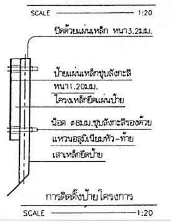
SCALE 1:20
