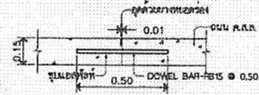
CONTRACTION JOINT 1:20
