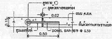
EXPANSION JOINT 1:20
